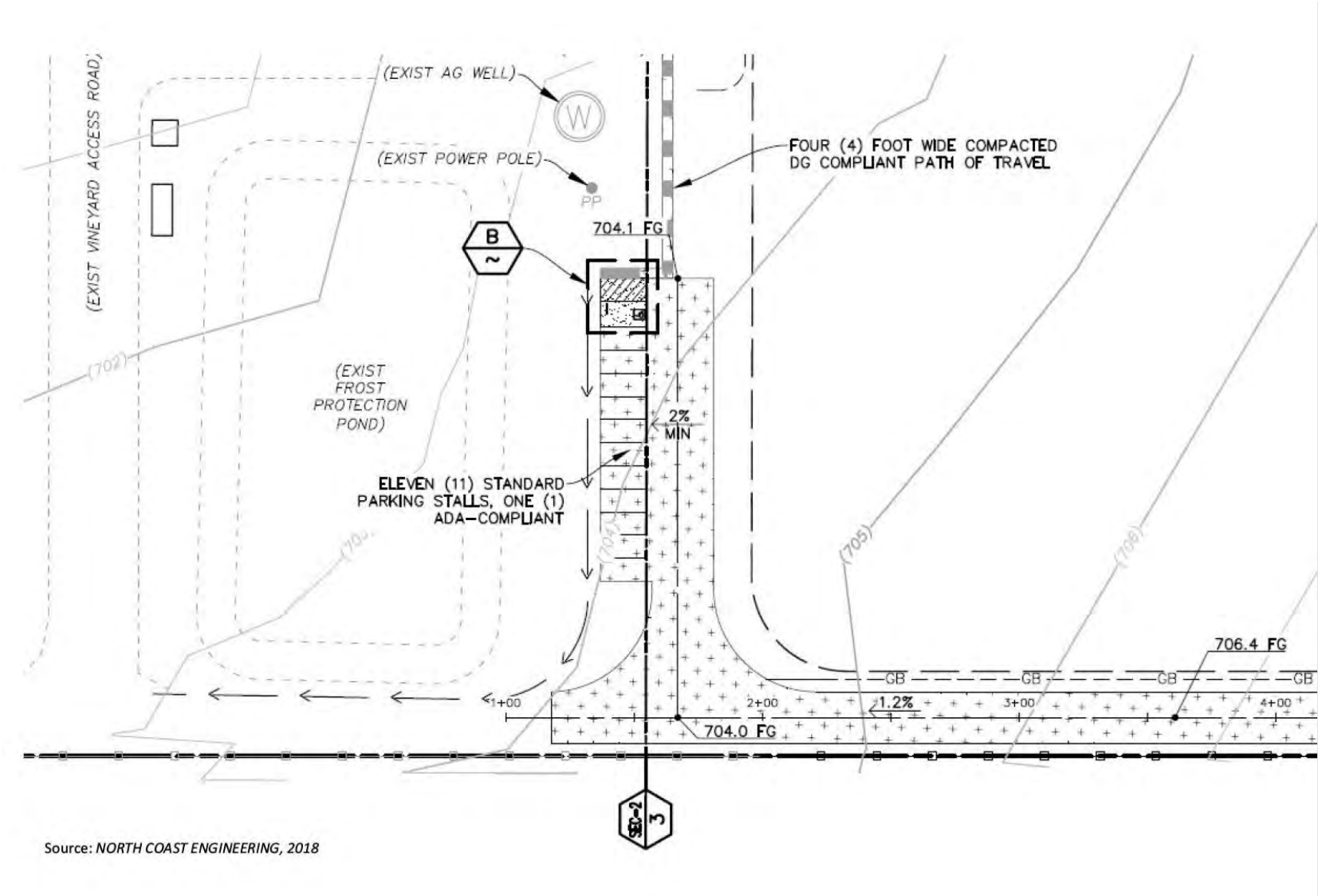
Figure 4 – Proposed On-site Parking
